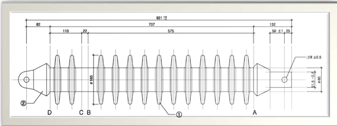
[Long Rod Insulator]
